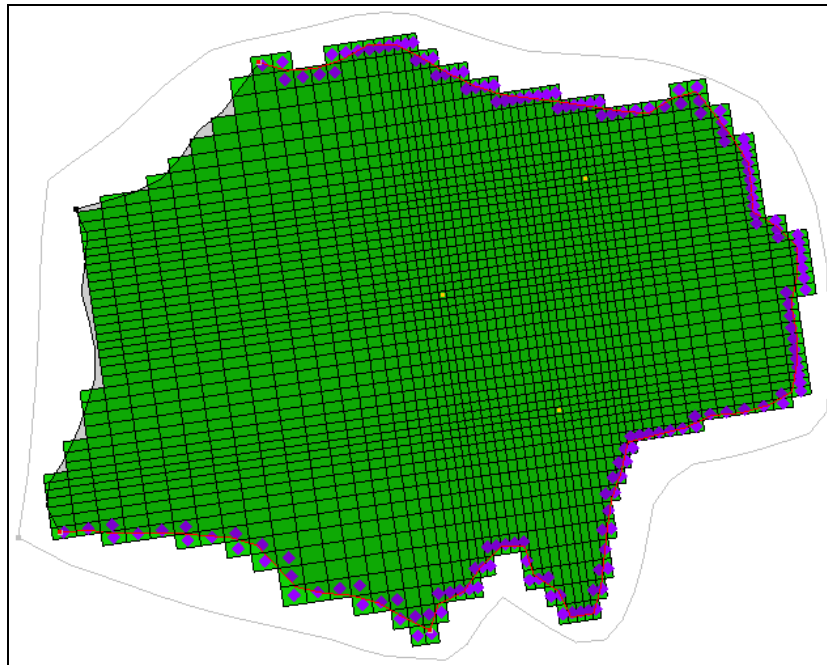
Figure 15 Plan view after map converted to MODFLOW
