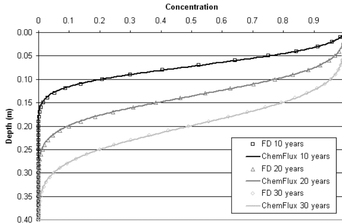
Figure 3 1D CHEMFLUX versus CONTAM.zip Diffusion, Advection, and Dispersion
