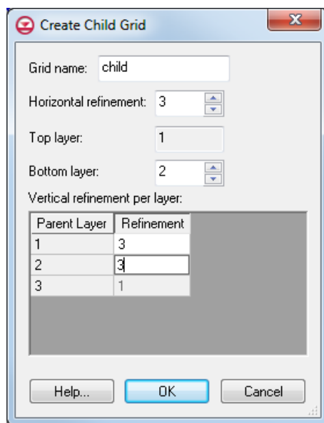
Figure 4 Create Child Grid dialog
