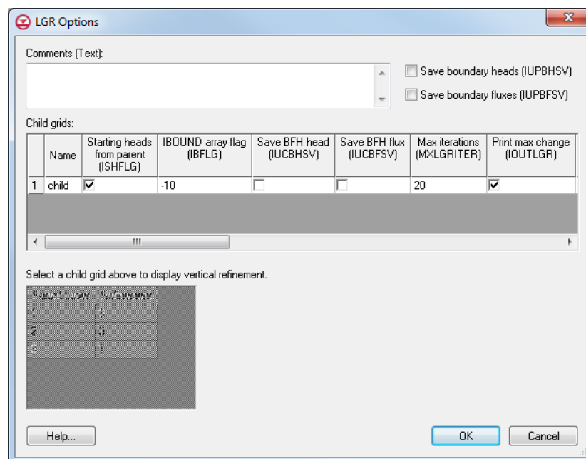
Figure 10 LGR Options dialog
