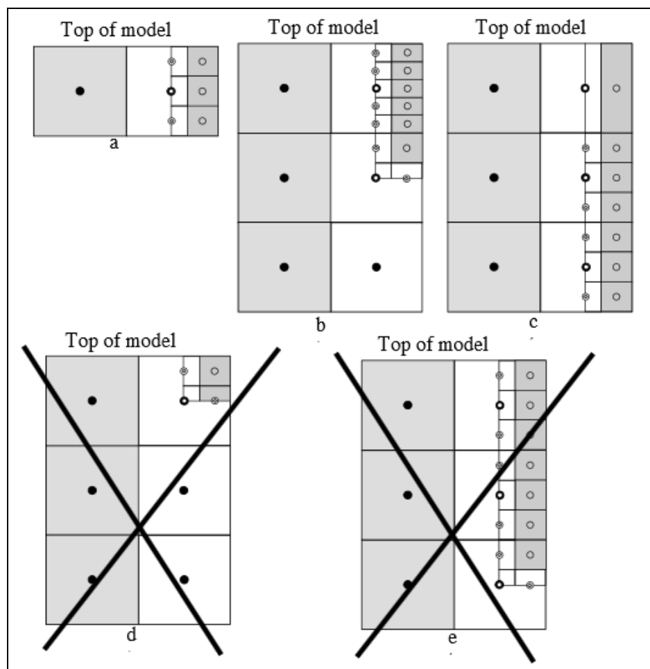
Figure 9 Vertical refinement rules 2
