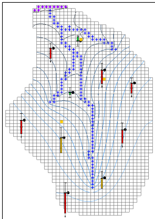
Figure 1 MODFLOW 2000 model
