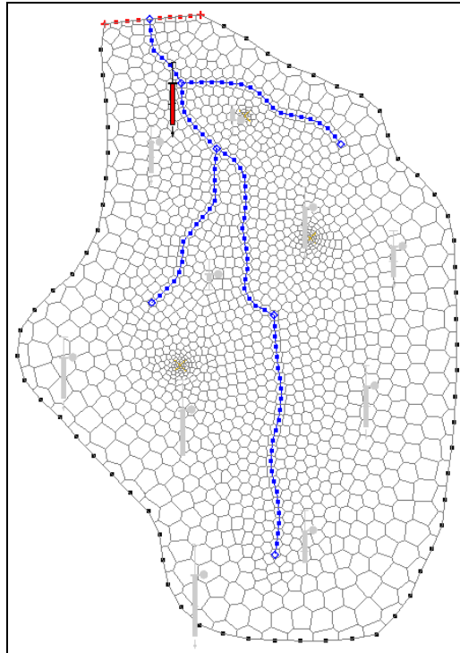
Figure 8 Voronoi UGrid
