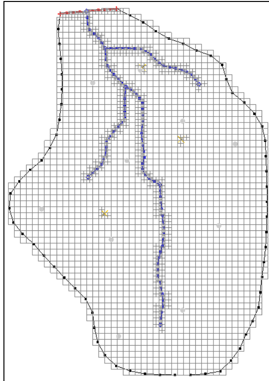
Figure 9 Quadtree UGrid
